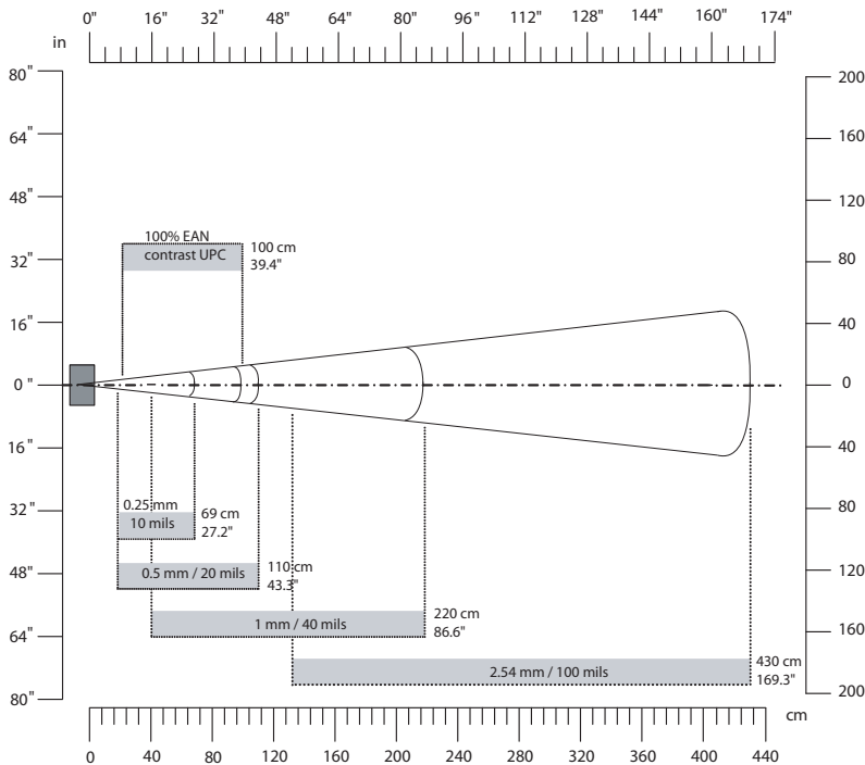
EX25B Near-Far Range Imager 1D Minimum Reading Distances: This graphic does not include the 0.24 cm (0.09 in) setback for the CK3.
