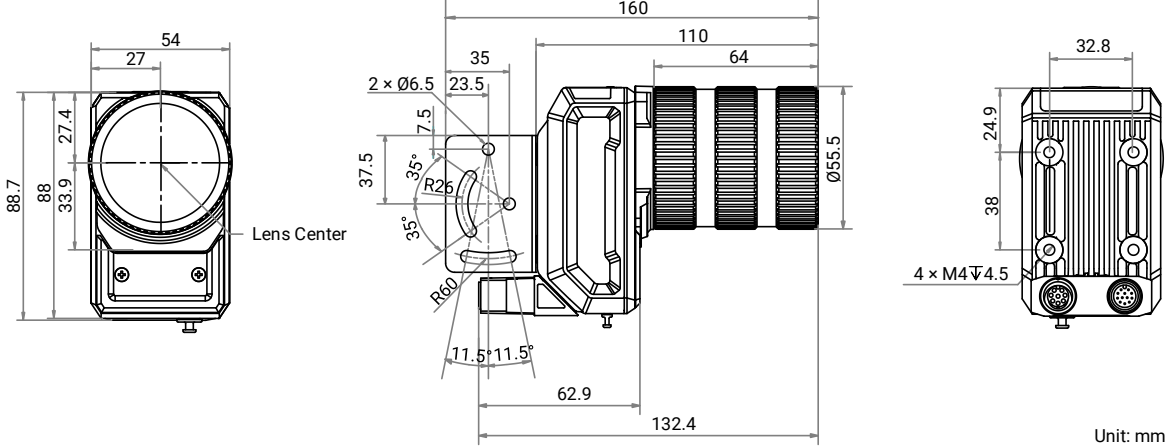
Installation Bracket:
