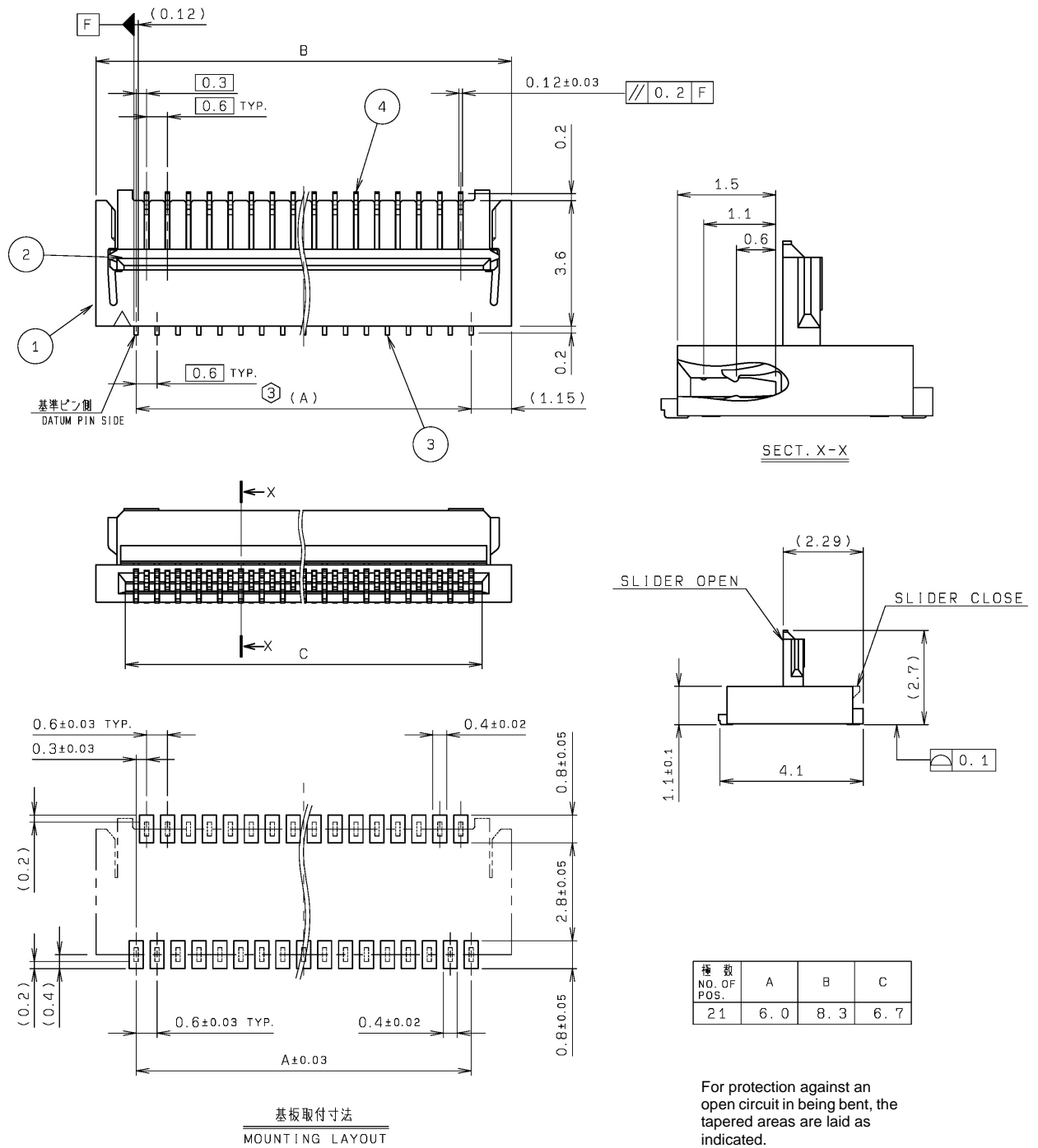
Figure 3-4 21-Pin ZIF Connector (SE3300 Imager to Flex), Kyocera 6283 Series
