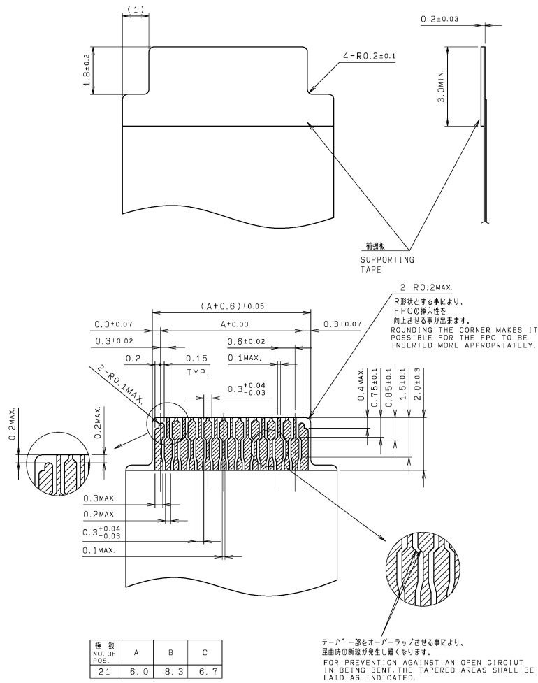
Figure 3-5 21-Pin ZIF Connector (SE3300 Imager to Flex), Kyocera 6283 Series (continued)
