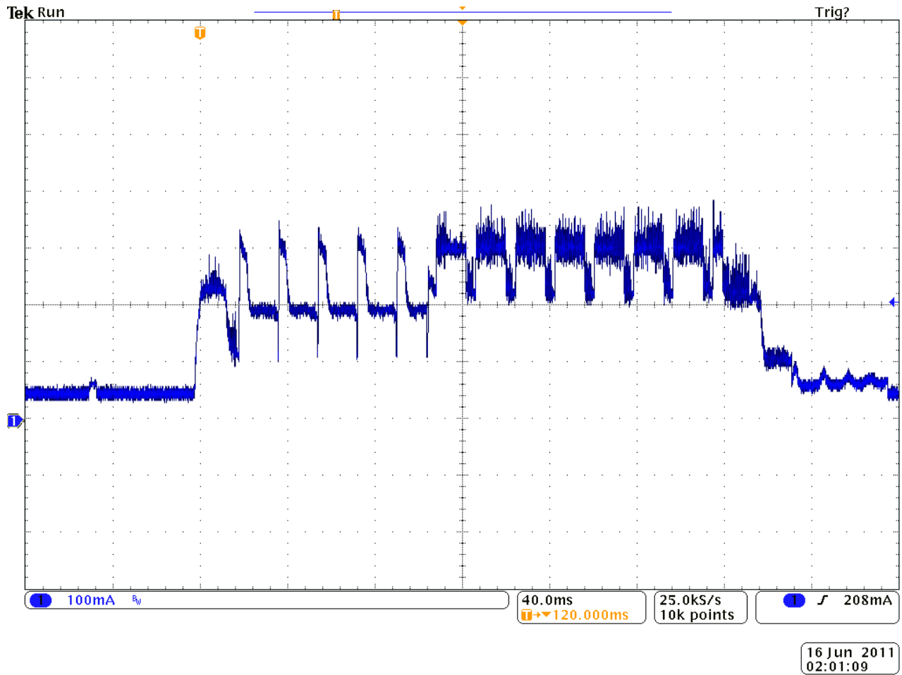
Figure 2-3 PL3307 Supply Current - 3.3 V Operation (RS-232, SSI, Scan/Decode Session)
