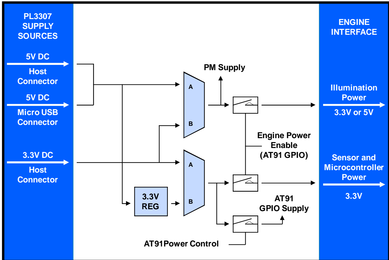
Figure 2-2 PL3307 Power Supply Multiplexer
