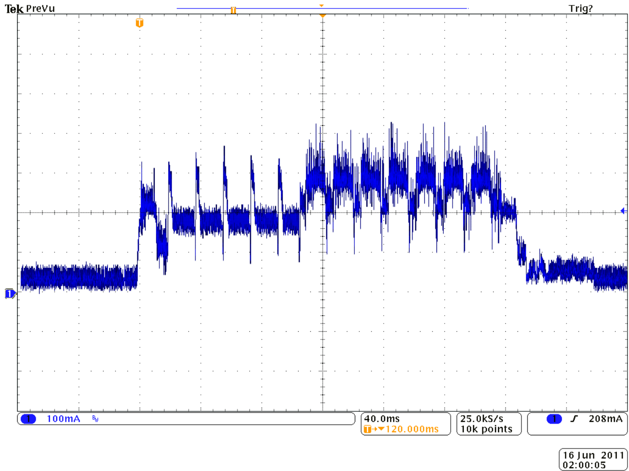
Figure 2-5 PL3307 Supply Current - 5 V Operation (USB Self Powered, Scan/Decode Session)
