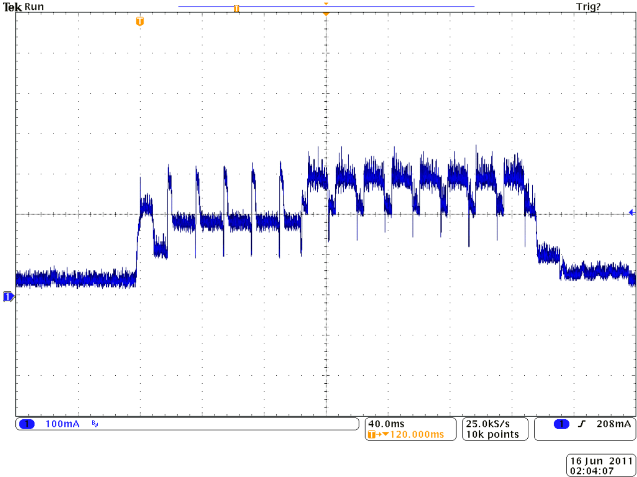
Figure 2-4 PL3307 Supply Current - 5 V Operation (USB Bus Powered, Scan/Decode Session)
