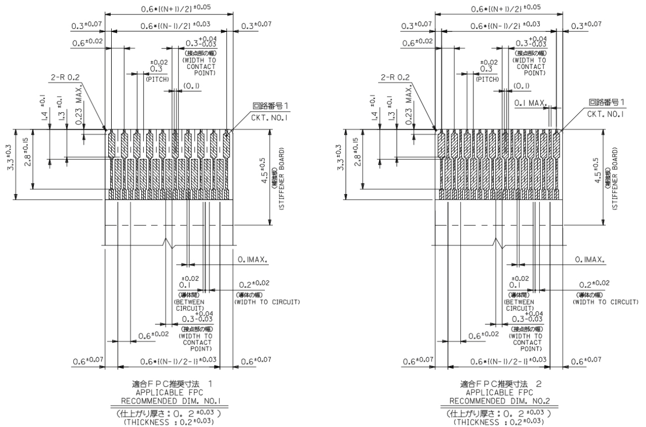
Figure 3-2 21-Pin ZIF Connector (PL3307 Decoder to Flex), Molex 54809 Series (continued)
